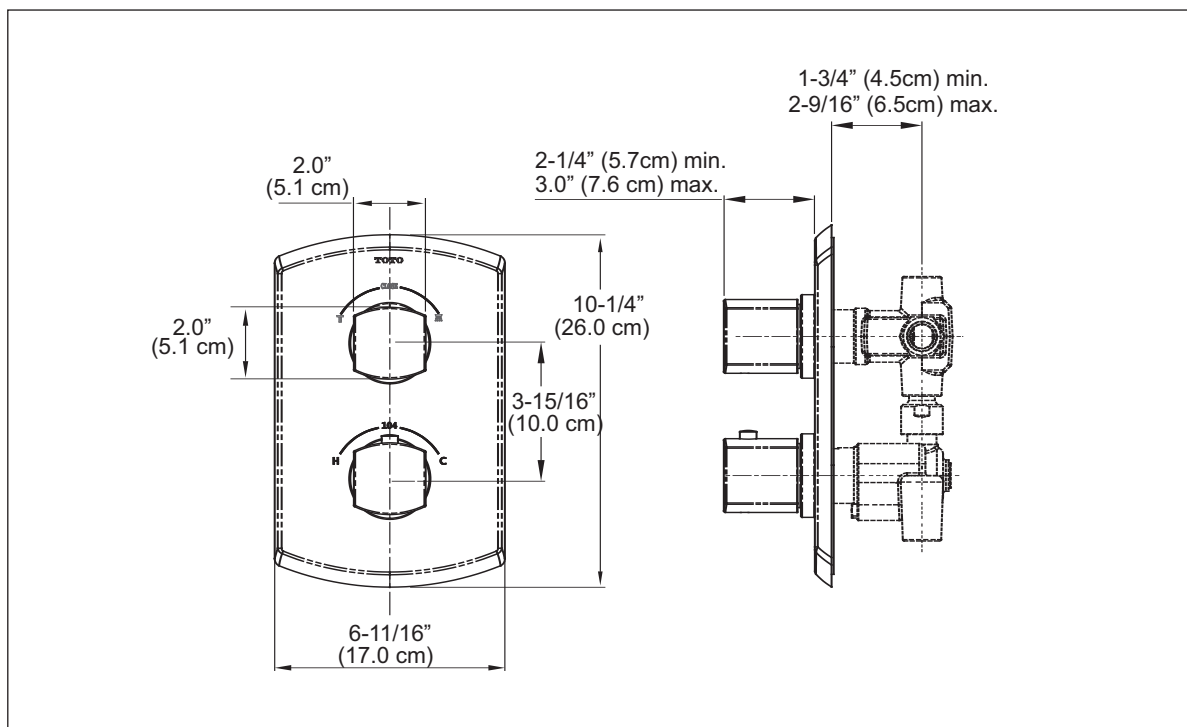
TS960DC - Soirée™ Thermostatic Mixing Valve Trim with Dual Volume Control
