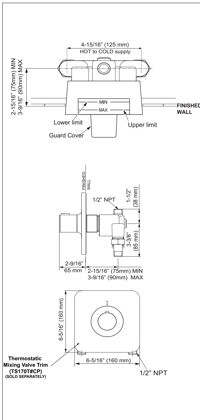
TSKT - SMA Thermostatic Mixing Valve
