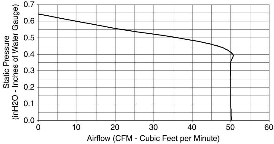
XN50 - 4" DUCT
