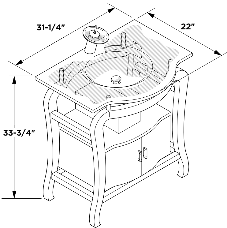
Vanity Front
