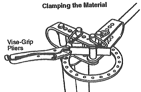
Clamping the Material
