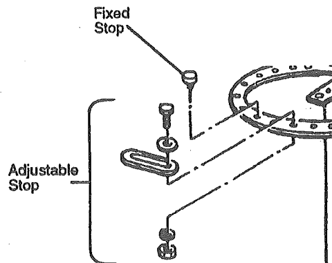
Fixed and Adjustable Stops
