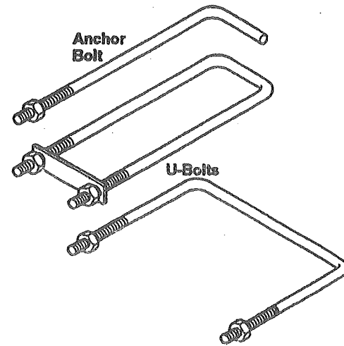
TYPICAL U-BOLTS AND ANCHOR BOLTS
