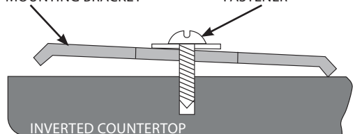
INVERTED COUNTERTOP
