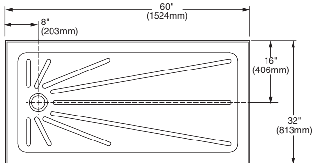
6032S1.STL.020 Left Hand Drain
