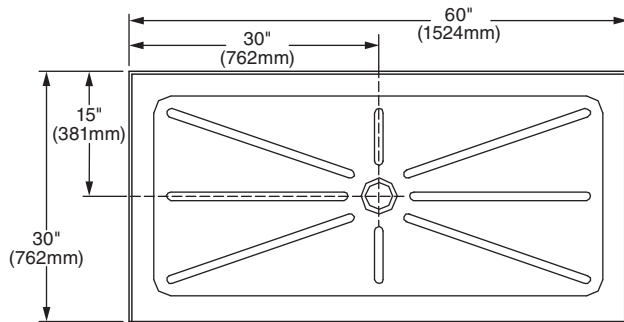
6030S1.STC.020 Center Drain
