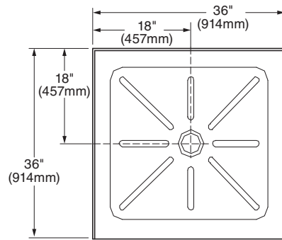
3636S1.ST.020 Center Drain
