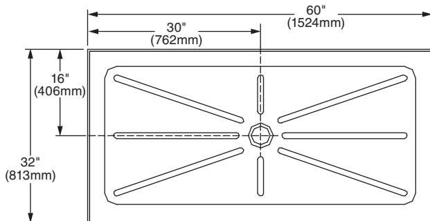
6032S1.STC.020 Center Drain
