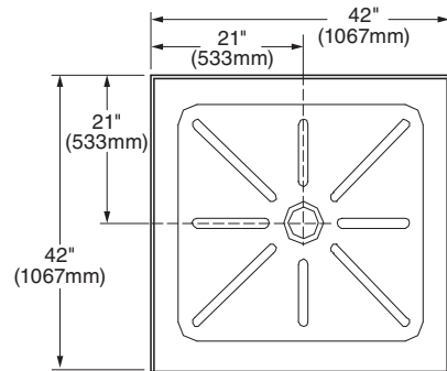
4242S1.ST.020 Center Drain
