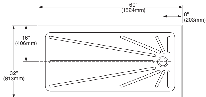
6032S1.STR.020 Right Hand Drain
