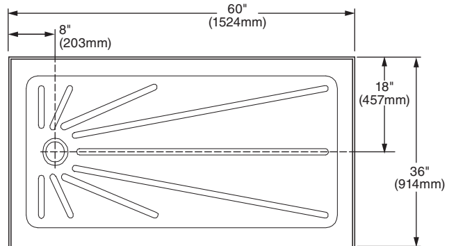
6036S1.STL.020 Left Hand Drain
