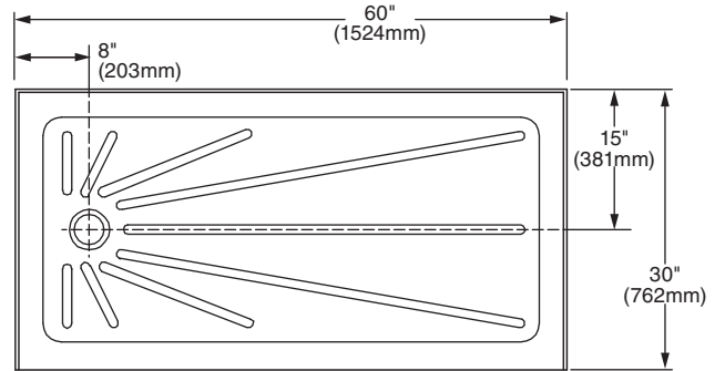
6030S1.STL.020 Left Hand Drain
