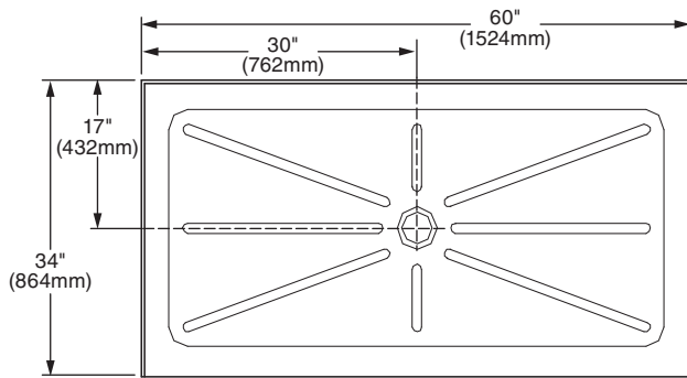
6034S1.STC.020 Center Drain
