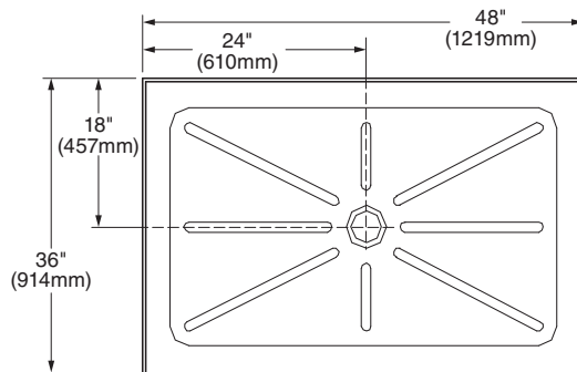
4236S1.ST.020 Center Drain
