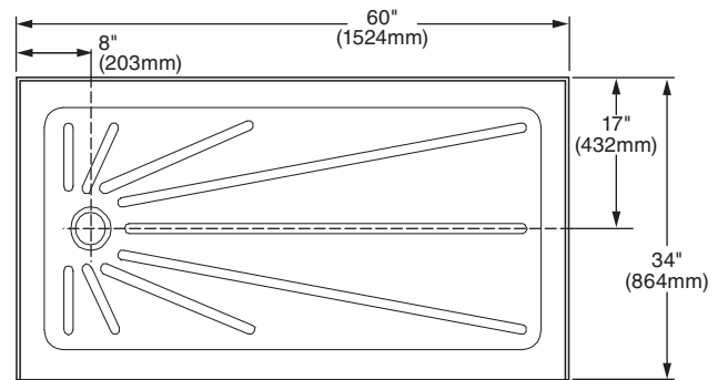
6034S1.STL.020 Left Hand Drain
