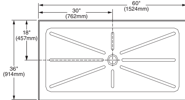
6036S1.STC.020 Center Drain
