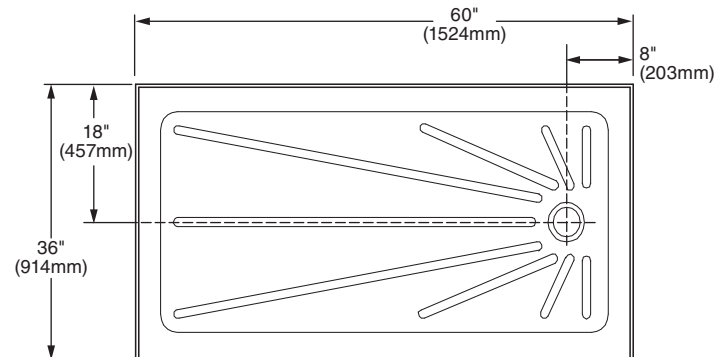
6036S1.STR.020 Right Hand Drain
