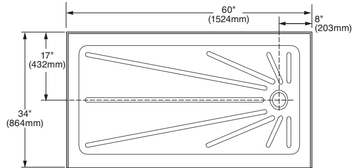
6034S1.STR.020 Right Hand Drain
