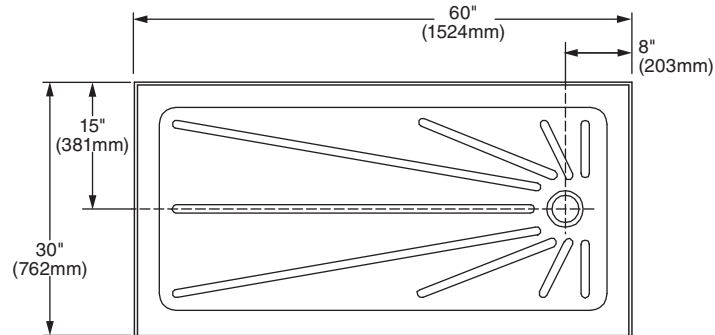
6030S1.STR.020 Right Hand Drain
