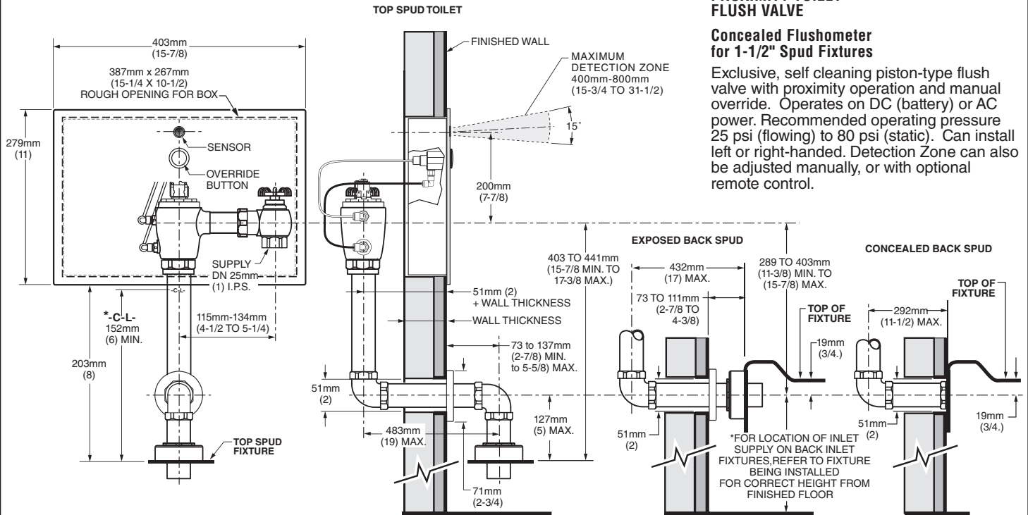
Fig. 1 Roughing-in Dimensions
