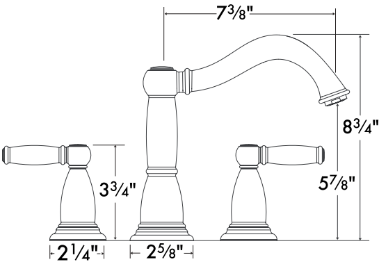
Tango - lever handles shown
