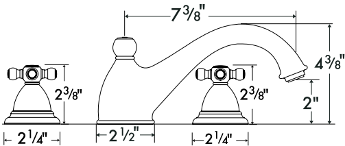
Limbo - cross handles shown
