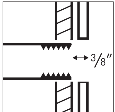
Installation with 3/4" NPT female fitting
