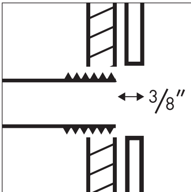
Installation with 1/2" NPT male nipple
