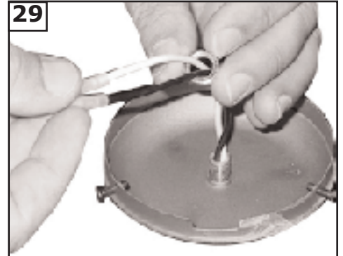
Install keeper nut over lead wires.
