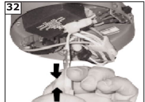
Locate blue and white wire from the fan marked "For light kit". Connect blue from fan to black from light and white from fan to white from light by pushing connectors together.
