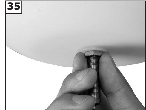
Attach the glass to the light fixture. Install the rubber washer first and then the hex nut to the glass to secure in place.
