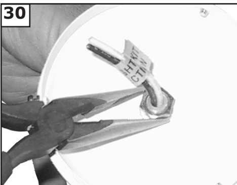
Tighten keeper nut onto threaded pipe from the light kit.
