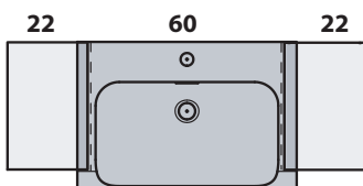
= 100 cm CENTRATO / CENTERED WASHBASIN
