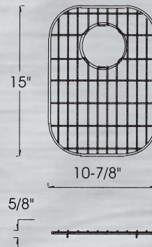
Model: BG4233 Bottom Grid for MAG503, MAG1815, MAG505, MAG8503L
