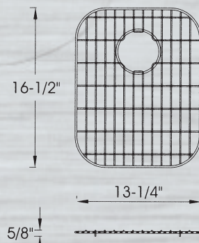
Model: BG4740 Bottom Grid for MAG503, MAG504, MAG 8503L
