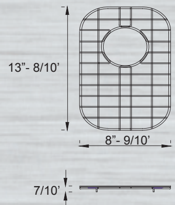
Model: BG4026 Bottom Grid for MAG3121L, MAG3320
