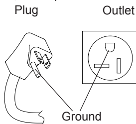
Figure 1: Plug and outlet configuration for 240 Volt, 20 Amp circuit
