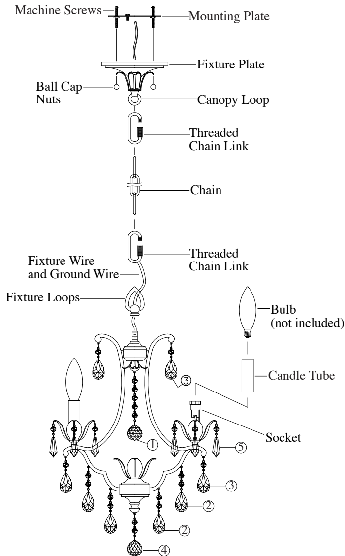
FIG: 1 CHAIN HUNG INSTALLATION
