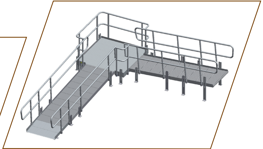
5' x 5' 90° Turn
