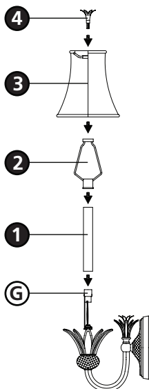
Drawing 3 - Fixture Assembly
