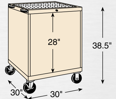
Model 63359 Usable height 28"
