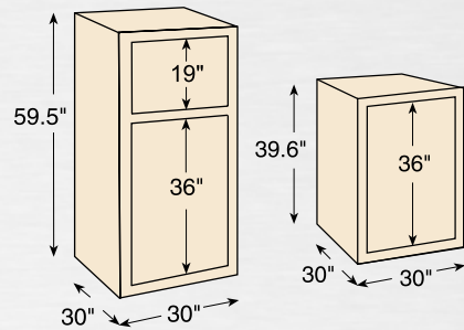
Housing No. 63600 Usable Height 55" Housing No. 63400 Usable Height 36"
