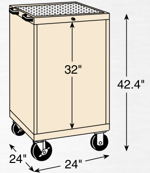
Model 61759 Usable height 32"
