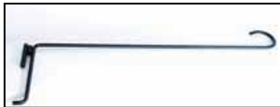
SP15 Flag Mount Bracket 25"D X 8"W X .5"H Wt. 0.9078 lbs./Case 4 7 15038 31060 0
