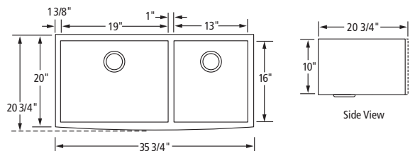
CPAZ3621-D10/10 Grid not available
