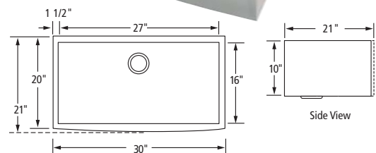
CPAZ3021-D10 Grid not available
