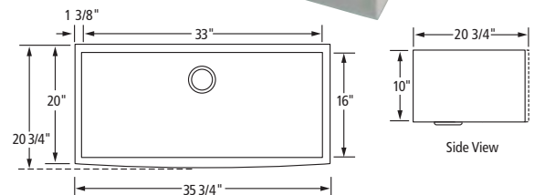
CPAZ3621-D10 Grid not available
