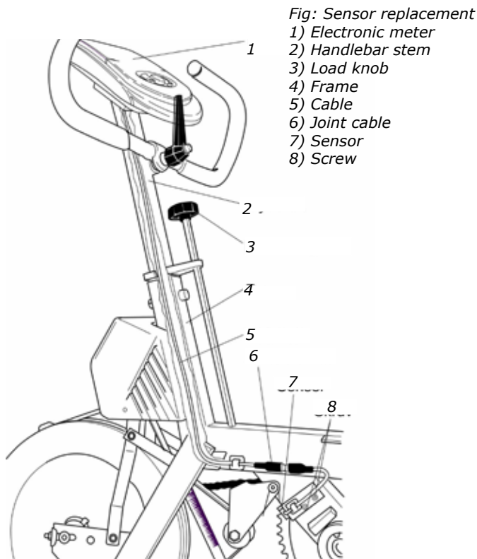
Fig: Sensor replacement
