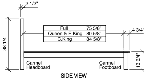
Assembled Product and Carton Dimensions *
