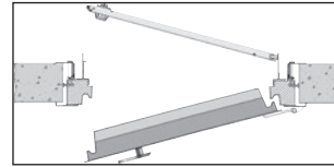
Right Swing Vault Door – Left Swing Daygate
