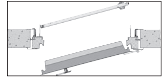
Right Swing Vault Door – Right Swing Daygate
