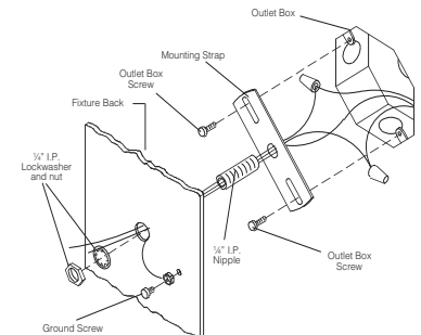
Figure 2: Wall mount
