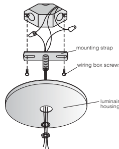
Figure 1: Ceiling mount
