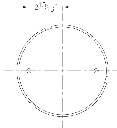
Figure 3: Secondary Wall Mount Screw Holes
