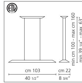
Float L ceiling / suspension
