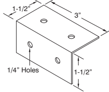
Mounting Bracket View
