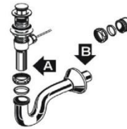
Typical Drain Assembly
