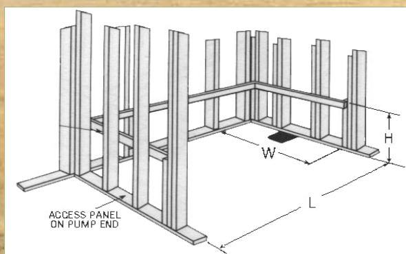
Framing Dimensions
