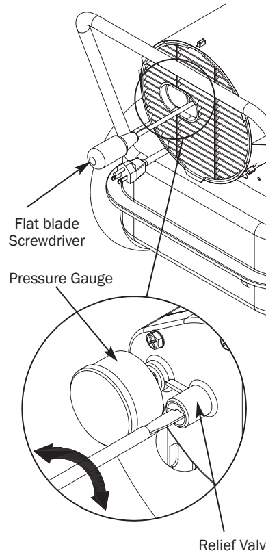
Figure 18 – Adjusting Pump Pressure
