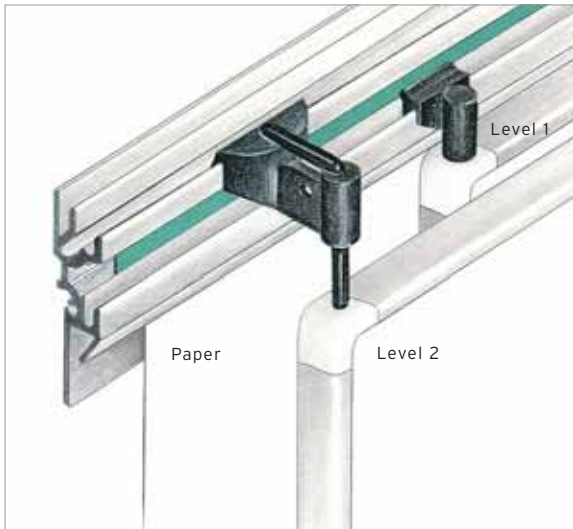
MODEL 7705 WALL TRACK (with integrated display rail) Slide sheet under rollers to insert
