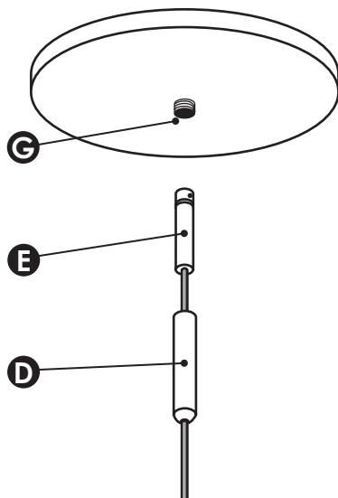
Diagram shows Canopy C-8120 with a cable assembly.
