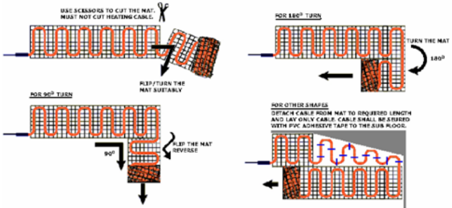
Illustration of how to cut and lay your floor Heating Mats to suit your floor plan to cut and lay your floor Heating Mats to suit your floor plan
