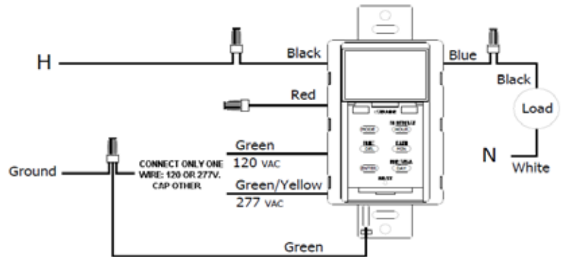
Wiring Diagram: Installation S700Z
