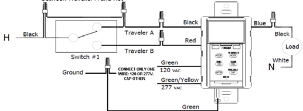
Wiring Diagram: Three-Way Installation S700Z
