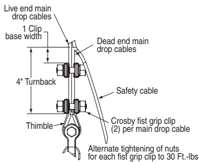
Detail D (See "preparing cable terminations", pg. 2 of TorkStar TS1000 or TS1400 instructions)
