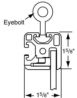
Large Screen Mounting Detail (90" diagonal and Larger)
