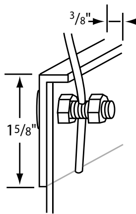
Standard Mounting Detail (Through 84" diagonal)
