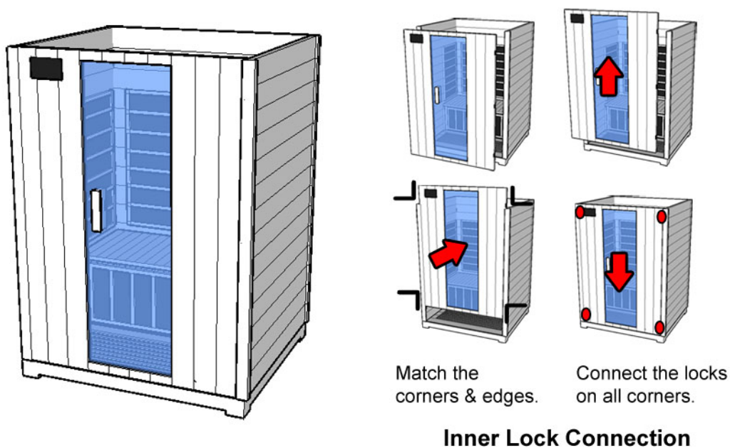
Figure C-5: Front Panel
